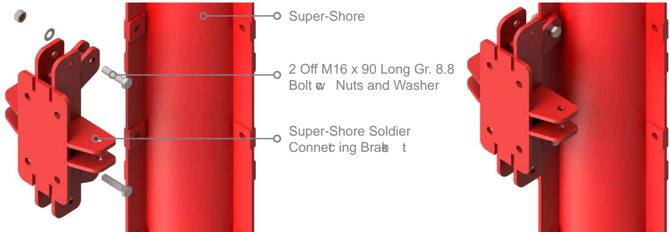
Super-Shore Soldier Connecting Bracket Connection To Super-Shore
